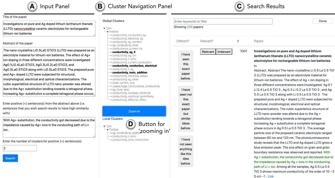
Figure 2: Front-end interface. A In the input panel, searchers enter the query paper abstract and a specific sentence aspect they want to align the retrieval results on. B Once searchers click on ‘Search’ at the bottom left, the system retrieves papers along with global domain clusters and displays them at the top of the navigation panel. Searchers can switch between different clusters to examine the results. Clicking on a cluster label highlights it and filters the papers that belong to the cluster in the table (clicking again on a selected cluster label de-selects it and refreshes the filtered table view). C The papers are displayed in the table on the right, with a green sentence highlight showing the closest aspect to the query. Searchers can type keywords in the filter at the top to find papers that contain them (matching keywords in the abstract are highlighted). Optional control buttons for our case studies for collecting feedback data are also shown in the table. D Clicking the ‘Zoom in’ button retrieves more papers from the selected clusters, allowing searchers to examine nuanced differences within the selected domain clusters.
