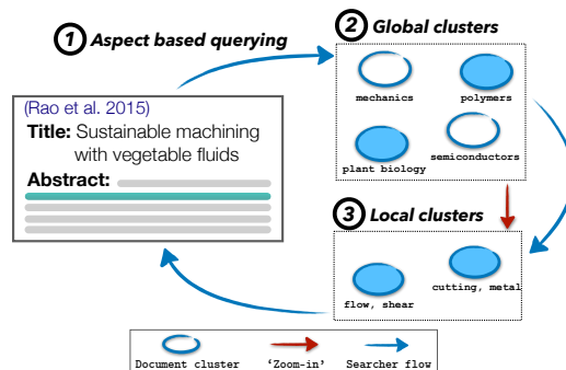
Figure 1: We leverage free-form sentence level querying ① to retrieve documents across automatically built domain clusters ②. These are expanded based on searcher selection and re-clustered to allow navigation of nuanced differences within selected global clusters ③. Searchers can move between global clusters, ‘zoom in’ to examine global clusters, and reformulate their queries for additional alternative exploration.
